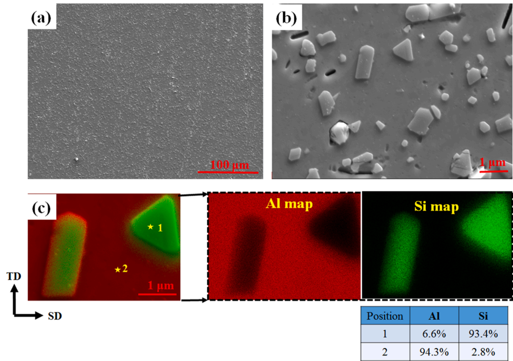
Fig. 7. SEM images of the ST specimen after chemical etching. (a, b): SEM images with a low and high magnification showing the distribution of silicon. (c) EDS element maps of the Al (red) and Si (green) for an area in (b).
