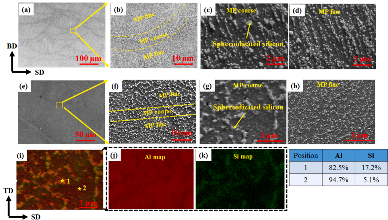
Fig. 6. SEM images of the SR specimen after chemical etching. (a-d): SEM images with a low, medium, and high magnification showing the typical fish-scale patterns, melting pool (MP) boundaries, and hierarchical structure in the BD-SD surface. (e-h): SEM images of the microstructure in the TD-SD surface with different magnifications. (i-k): EDS element maps of the Al (red) and Si (green) for (g).
