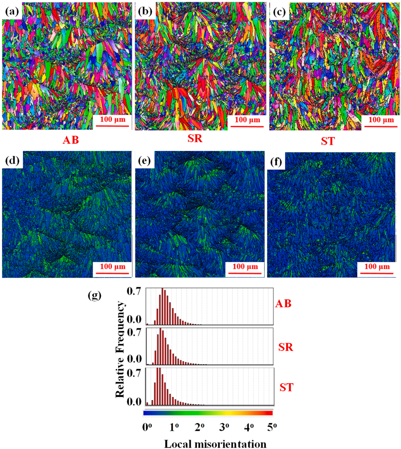
Fig. 8. IPF maps of the (a) AB, (b) SR, and (c) ST samples. Local misorientation map of the (d) AB, (e) SR, and (f) ST samples. (g) A comparison of the local misorientation histogram for the three samples.
