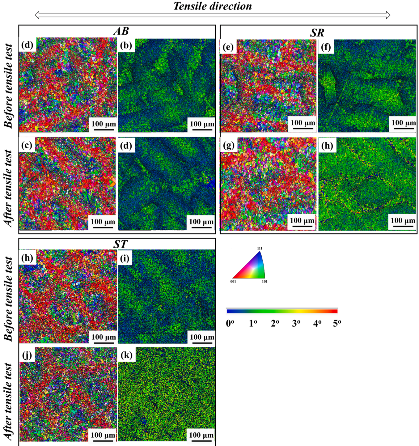
Fig. 9. Comparison of the microstructure and local misorientation distribution for the AB, SR, and ST processed AMed AlSi10Mg specimen before and after tensile tests.
