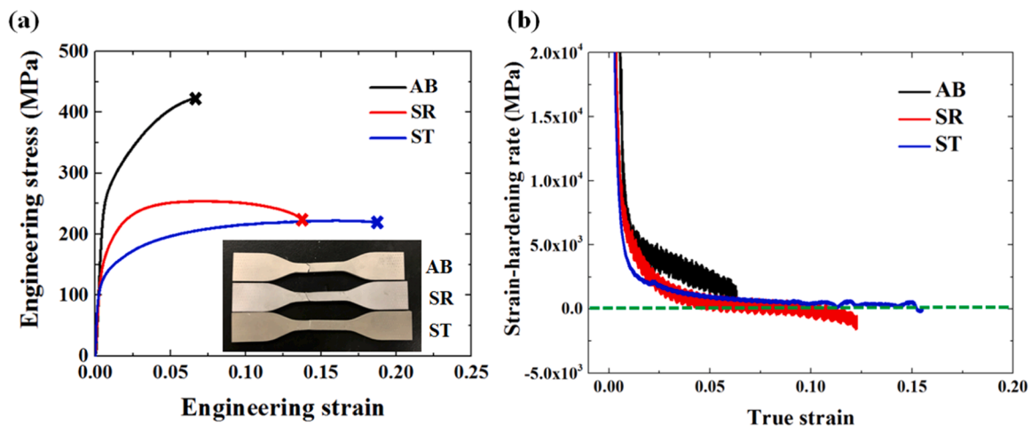
Fig. 2. (a) Engineering stress-strain curves of the AB, SR, and ST samples. The inserted figure shows the lengths of the three specimens after tensile tests. (b) Strain-hardening rates of the AB, SR, and ST processed AlSi10Mg samples during tensile tests.
