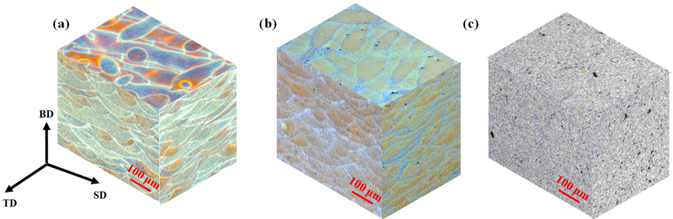
Fig. 4. 3D OM microscopy of the LPBF-fabricated AlSi10Mg specimen: (a) AB, (b) SR and (c) ST processed samples.
