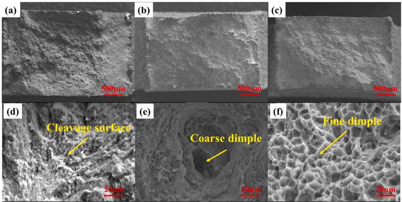
Fig. 3. SEM images of the fracture morphologies after tensile tests: (a) and (d) correspond to the AB samples; (b) and (e) correspond to the SR processed samples; (c) and (f) correspond to the ST processed samples. (a-c) are the SEM images of the fracture surfaces with a low magnification; (d-f) are the magnified fracture surfaces showing different fracture mechanisms.
