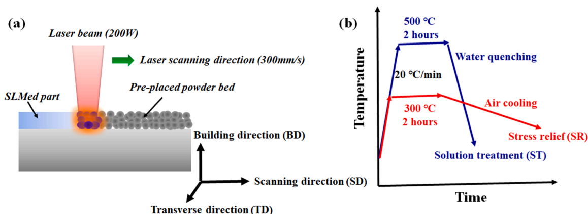
Fig. 1. Schematic illustration of the (a) LPBF process for fabrication of the AlSi10Mg alloy and (b) heat treatment routines for the ST and SR processes.
